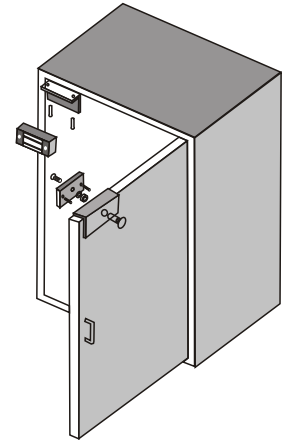
UL Bracket Installation
